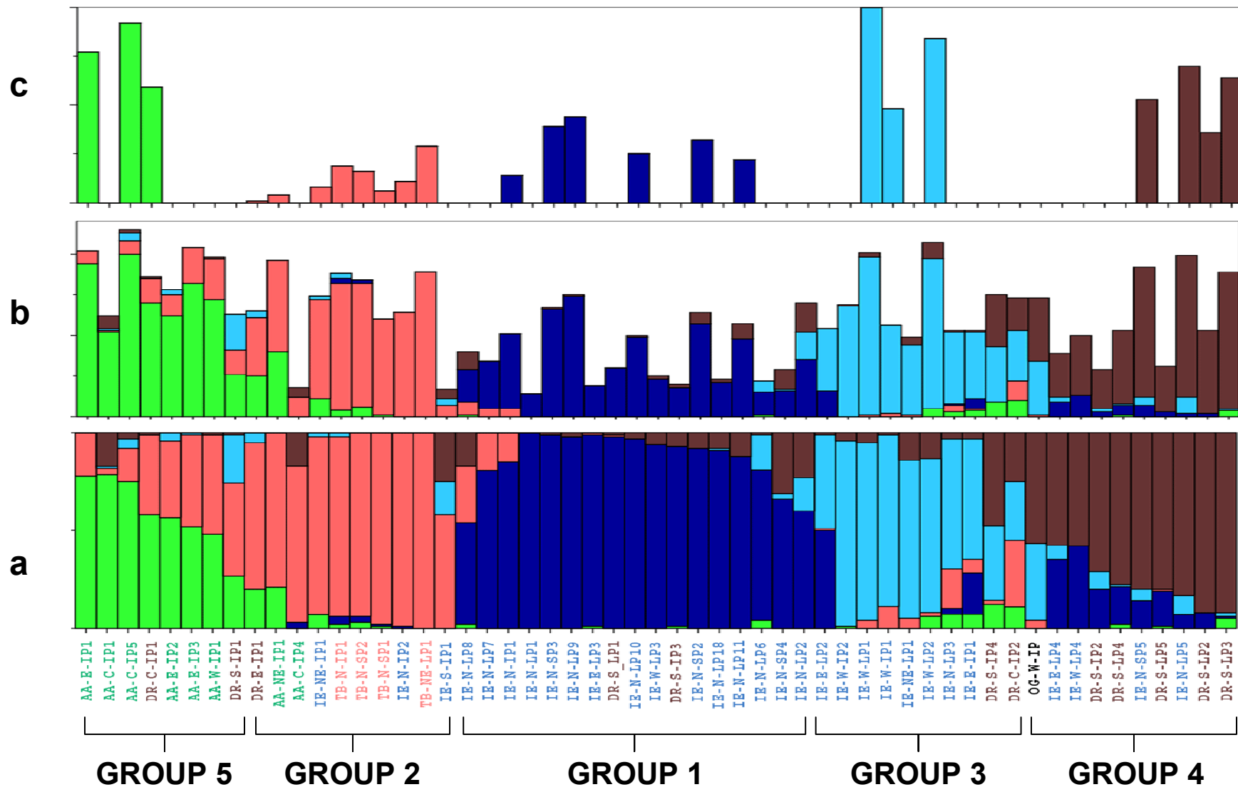
Supplementary Figure 2. Memberships of populations across clusters based on genotype frequencies of 405 SNPs. (a) Fuzzy, (b) Possibility and (c) Typicality measures of five clusters of populations are depicted. Fuzzy, differential membership of a population across clusters; Possibility, differential membership of a cluster across all populations relative to all population-cluster assignments; Typicality, differential membership of a cluster only across its core members.
